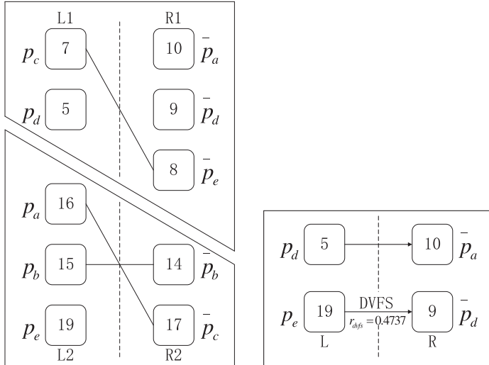
(c) A minimum cut is performed on \mathcal{G}_p , followed with the bipartite matching in each upper level block.
