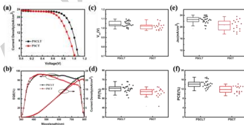
Figure 4. (a) The reverse-direction-scan J-V curves of the best-performance PSCs based on Li-treated TiO 2 and conventional TiO 2 , (b) EQE curves and integrated current density of different samples, (c)~(f) the V OC , FF, J SC , PCE versus two kinds of solar cells.
