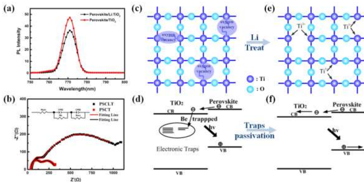
Figure 2. (a) Stable PL curves of perovskite films on Li-treated TiO 2 and conventional TiO 2 , (b) EIS Nyquist plots of the perovskite solar cells based on Li:TiO 2 and TiO 2 , (c) oxygen vacancies in TiO 2 lattice before passivation, (d) electronic traps below the conduction band in TiO 2 , (e) the Ti 3+ that exist in TiO 2 lattice after the Li-treating and (f) the energy diagram after traps have been passivated.
